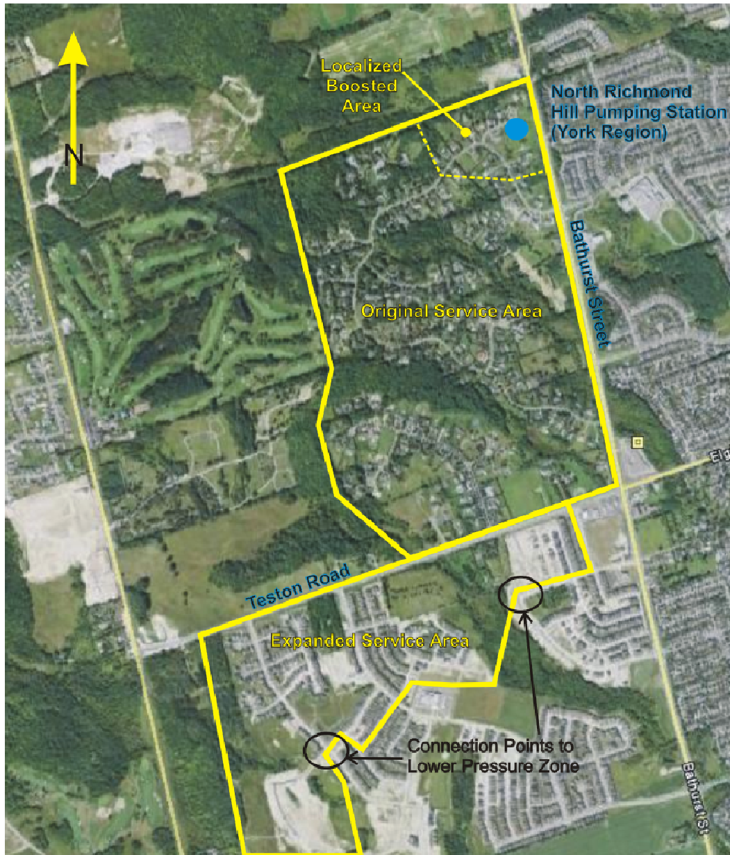
FIGURE 1. CITY OF VAUGHAN PD8 PRESSURE ZONE
